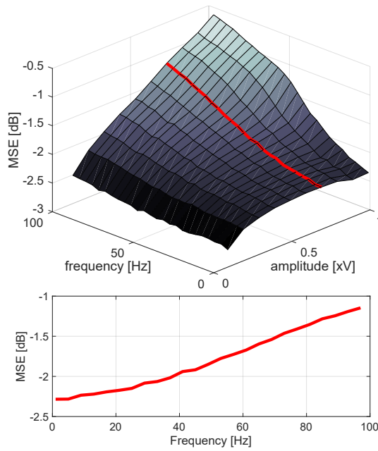
Figure 12. MSE of the tracking performance as a function of frequency (1 Hz to 100 Hz) and amplitude (0.1 V to 1 V), presented in decibels (dB). The red curve highlights the response of the system for a fixed amplitude of 0.7 V
