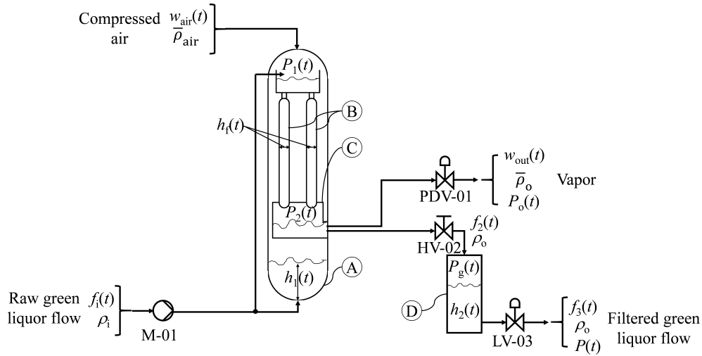
Figure 1. Process diagram of X-Filter process plant
