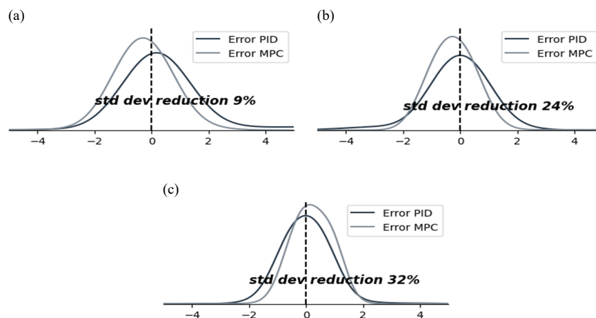
Figure 7. Probability density function of the standard deviation. (a) h_1 . (b) h_2 . (c) \Delta p
