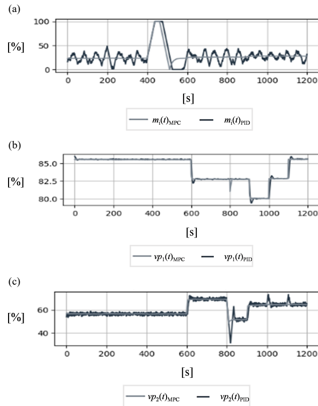
Figure 6. Simulation results of the manipulated variables, under transient. (a) m_i(t) . (b) v_{p1}(t) . (c) v_{p2}(t)
