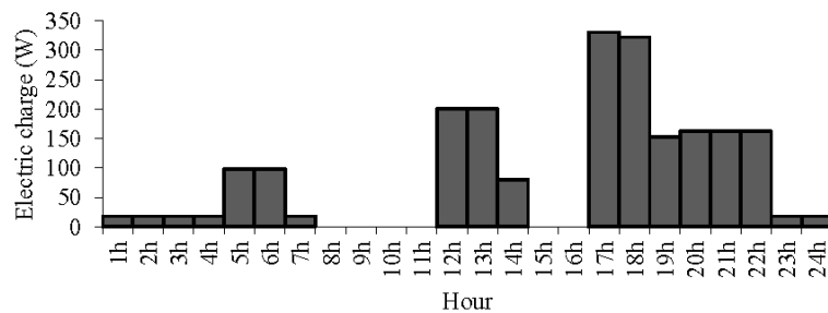
Figure 4. Average load profile for the 10 households surveyed (Source: authors' surveys)
