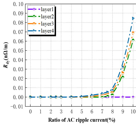
Figure 2. Distribution of dynamic resistance among layers with different ripple coefficients at the fixed power transmission distance L = 1 km
