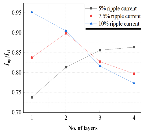
Figure 4. Normalized total current distributions among layers with different ripple coefficients at the fixed power transmission distance L = 1 km
