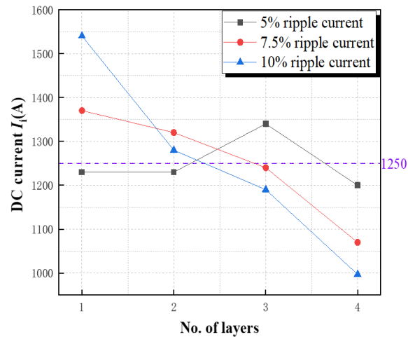
Figure 3. DC distribution among layers with different ripple coefficients at the fixed power transmission distance L = 1 km
