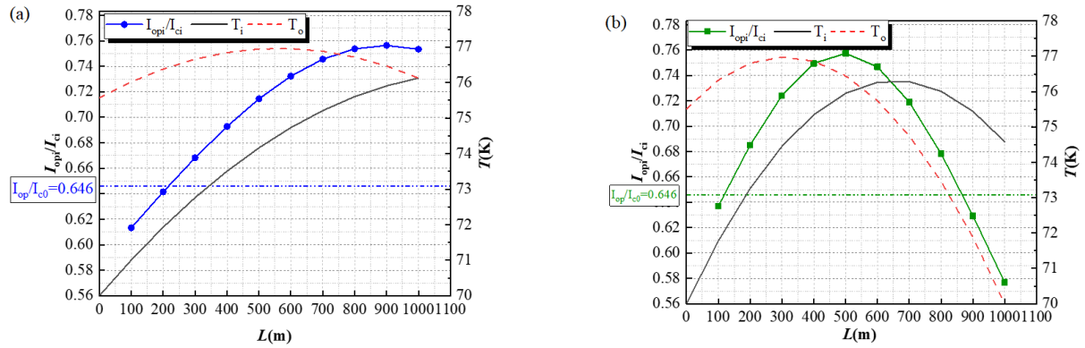
Figure 5. Variation of normalized operating current (left) and temperature (right) with the increasing transmission distance L (a) single refrigeration station (b) with sub-cooled stations
