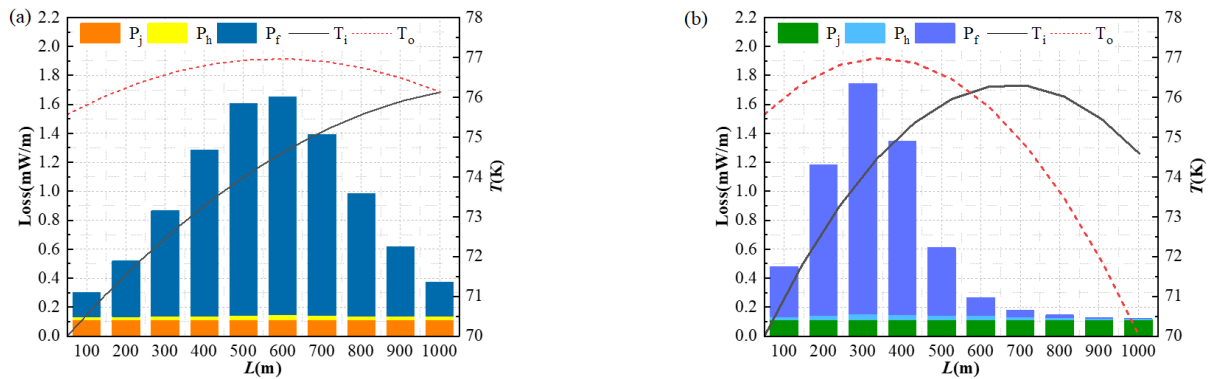
Figure 6. Different composition of AC losses and temperature with the increasing transmission distance L . (a) single refrigeration station (b) with sub-cooled station
