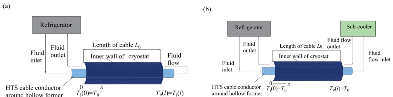
Figure 1. Counter-Flow cooling arrangement (a) single refrigeration station (b) with sub-cooled station
