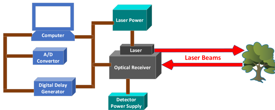
Figure 1. Schematic diagram of the Multi-wavelength Airborne Polarimetric LiDAR system (MAPL)
