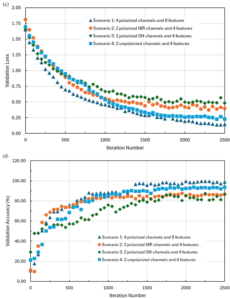
Figure 4. Training loss (a), training accuracy (b), validation loss (c) and validation accuracy (d) vs. iteration number during a typical run of the training or validation progress for SCENARIO 1, 2, 3 and 4 with 5 hidden layers in the feature extraction
