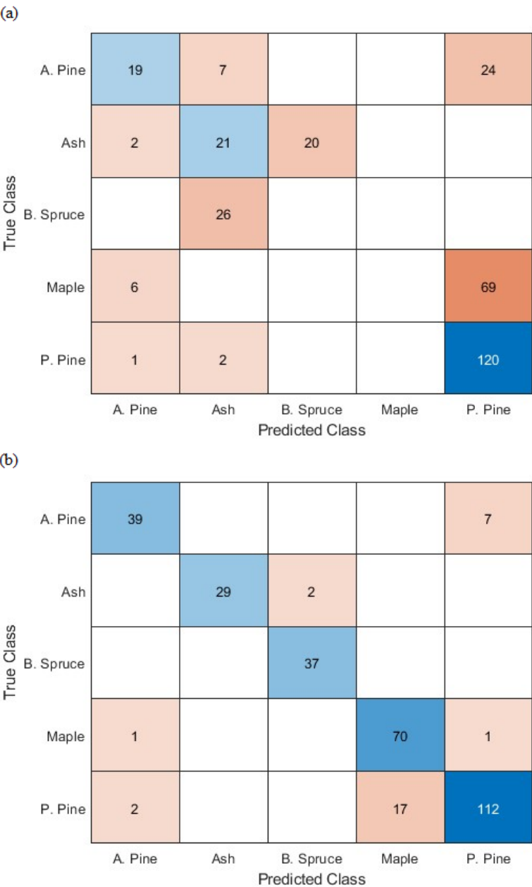
Figure 5. Confusion matrices of prediction (test) accuracy after training and validation processes for SCENARIO 3. (a) with 1 hidden layer and (b) with 5 hidden layers
