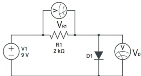
Figure 3. The forward-biased diode experiment circuit diagram
