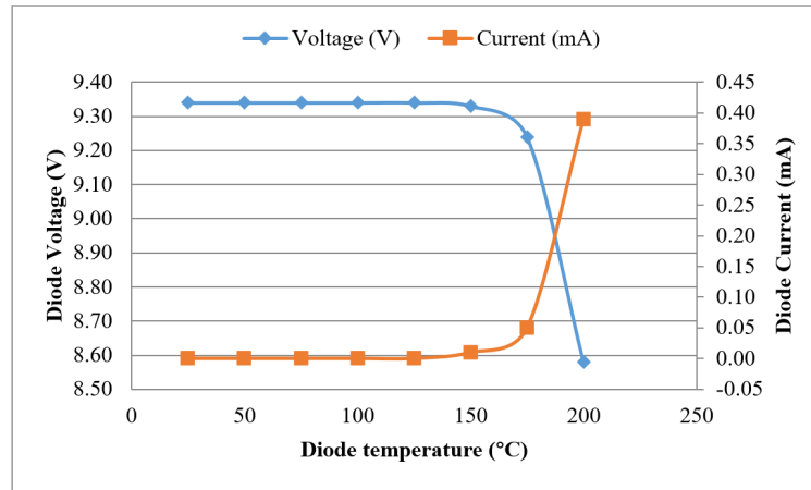
Figure 18. A graph of the reverse-biased IN5401 diode voltage and current against temperature
