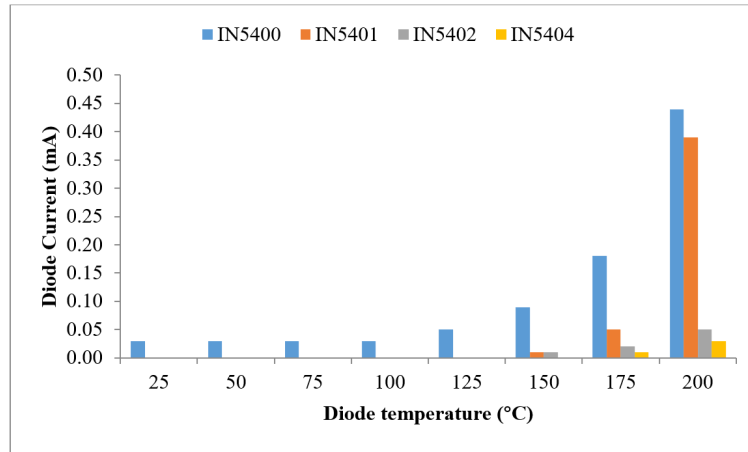
Figure 16. A bar chart of the reverse-biased diode current against temperature
