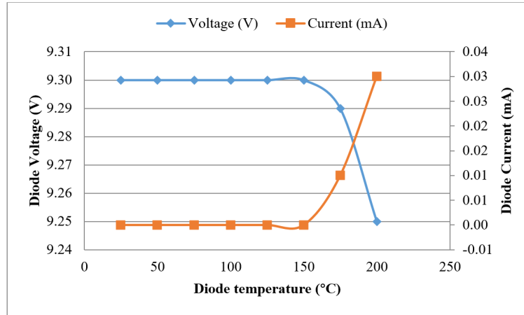
Figure 20. A graph of the reverse-biased IN5404 diode voltage and current against temperature
