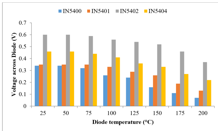
Figure 7. A bar chart comparing the forward-biased diodes' voltage against temperature
