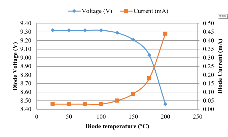
Figure 17. A graph of the reverse-biased IN5400 diode voltage and current against temperature
