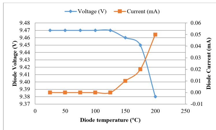
Figure 19. A graph of the reverse-biased IN5402 diode voltage and current against temperature
