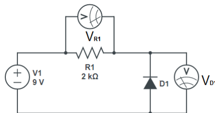
Figure 5. The reverse-biased diode experiment circuit diagram
