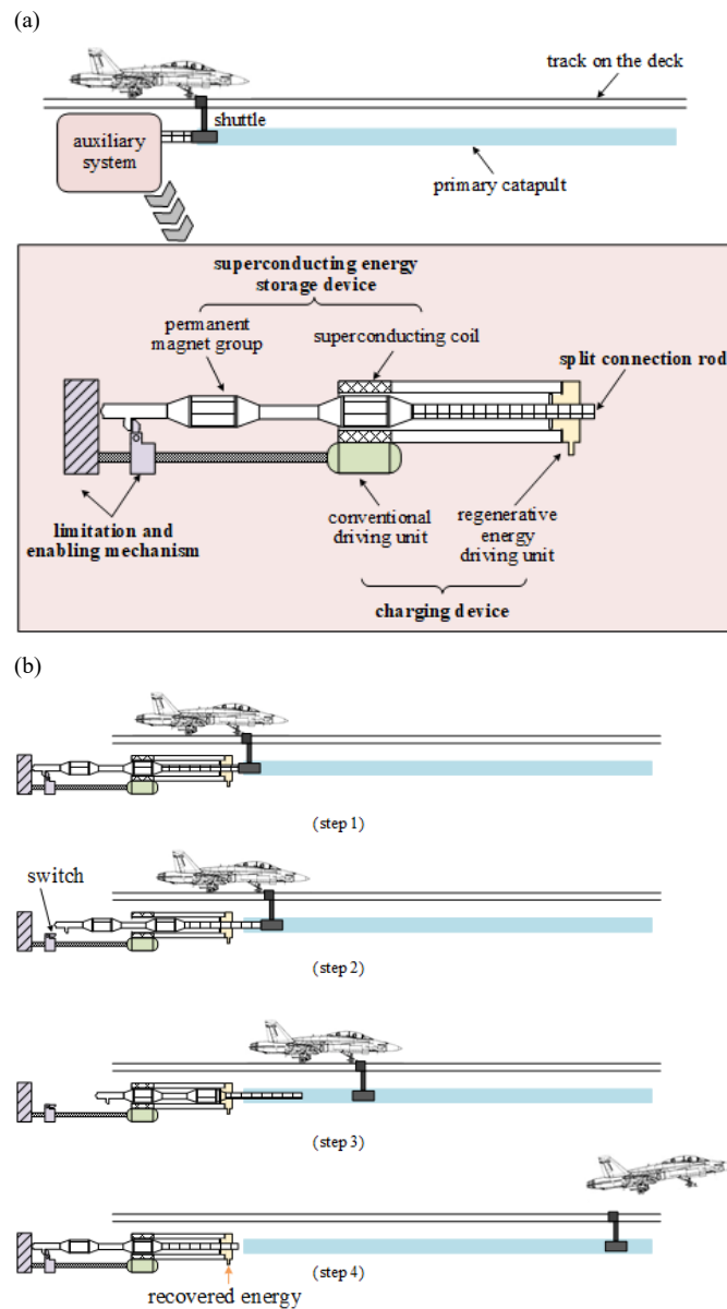
Figure 8. (a) Aircraft launch system equipped with the auxiliary system of the new energy storing/convert ing device, (b) operating process of the system [13]
