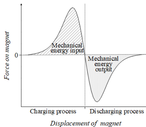
Figure 4. The energy storing/releasing cycle [10]
