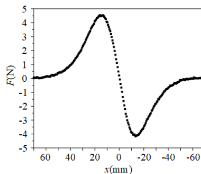
Figure 3. The interaction force on the magnet as a superconductor coil is used [1] (Note: x is the displacement of the magnet with respect to the origin, F is the interaction force between the magnet and superconducting coil.)
