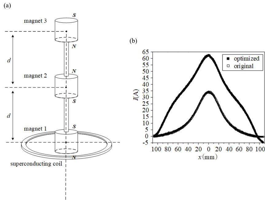
Figure 5. The optimized configuration and performance improving of the energy conversion/storage device [7, 8]. (a) Diagram of the optimized configuration, (b) The performance improvement (Note: x is the displacement of magnet 2 with respect to the origin.)
