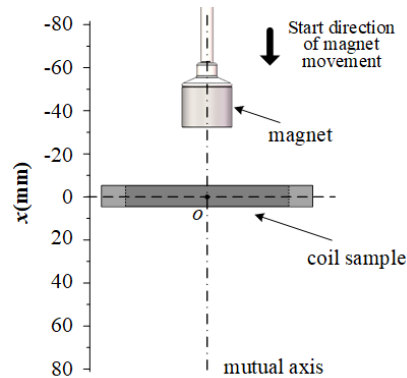
Figure 1. The configuration of a coil sample and a permanent (Note: 1. The coordinate origin is defined as the point of the geometric center of the coil sample; 2. x is the displacement of the magnet with respect to the origin.)
