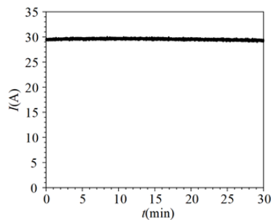
Figure 6. The current in the superconducting coil versus time as the magnet stopped at the origin [10] (Note: t is the time from the energy storage is completed, I is the current in superconducting coil)
