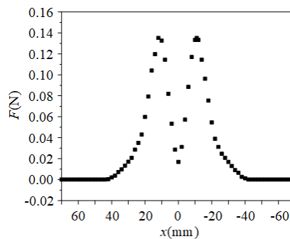
Figure 2. The interaction force on the magnet as a normal conductor coil is used [1] (Note: x is the displacement of the magnet with respect to the origin, F is the interaction force between the magnet and normal conductor coil.)
