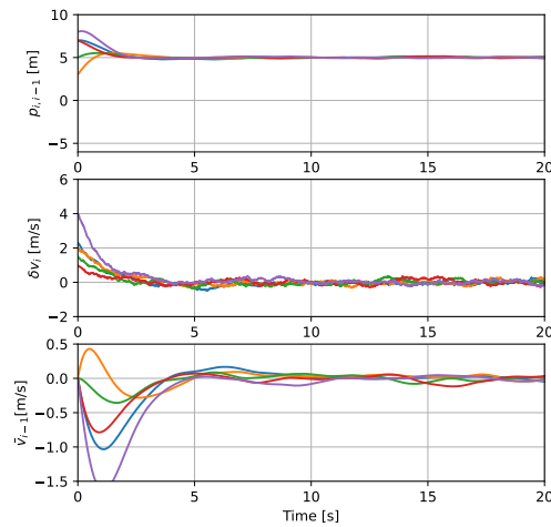
Figure 3. Trajectories of the intervehicular distance p_{i,i-1} , the velocity error \delta v_i and the estimation error \bar{v}_{i-1} for i \in \{1, 2, 3, 4, 5\}
