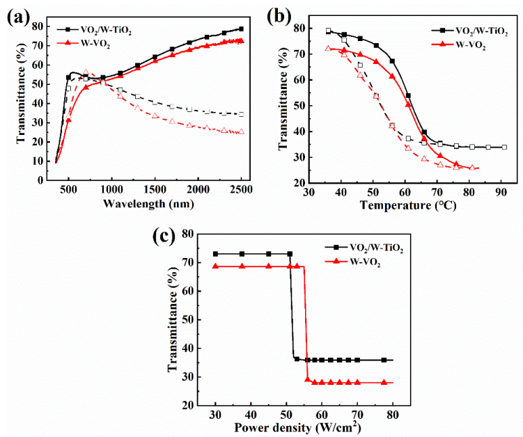
Figure 8. The comparison of phase transition performance between the VO_2/W-TiO_2 heterojunction and W-doped VO_2 film: (a) The transmittance spectra within 350-2,500 nm. (b) The hysteresis curves of the transmittance at 2,500 nm during heating and cooling processes. (c) The variation of the transmittance at 1,993 nm
