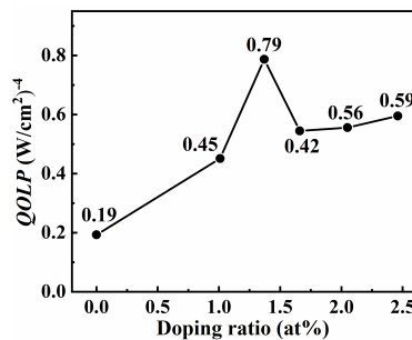
Figure 9. The QOLP of the VO_2/W-TiO_2 n-n heterojunction
