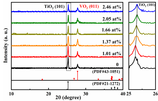
Figure 2. The XRD patterns of the VO 2 /W-TiO 2 heterojunctions
