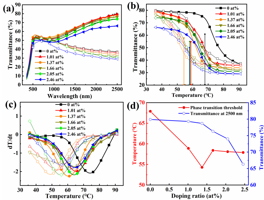
Figure 5. The effect of W doping concentration on the thermotropic phase transition performance of the VO 2 /W-TiO 2 heterojunction: (a) The transmittance spectra of the VO 2 /W-TiO 2 heterojunction in the wavelength range of 350-2,500 nm. (b) The hysteresis curves of the transmittance at 2,500 nm of the VO 2 /W-TiO 2 heterojunction during heating and cooling processes. (c) The first-order derivative curves of the hysteresis curves in Figure 5b. (d) The effect of W doping concentration on the T_c and t_M of the VO 2 /W-TiO 2 heterojunction
