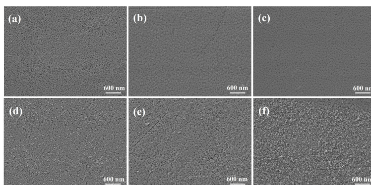
Figure 3. The effect of W doping concentration on the surface morphology of the \text{VO}_2/\text{W-TiO}_2 n - n heterojunction: (a) 0 at%; (b) 1.01 at%; (c) 1.37 at%; (d) 1.66 at%; (e) 2.05 at%; (f) 2.46 at%
