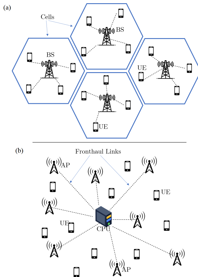
Figure 1. (a) Cellular MIMO, (b) Cell-Free MIMO
