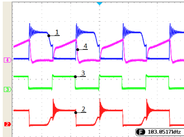
Figure 9. C-DC converter primary side experimental verification. 1 – Q1 Drain-Source voltage; 2 – D1 voltage; 3 – PWM; 4 – Q1 Drain current
