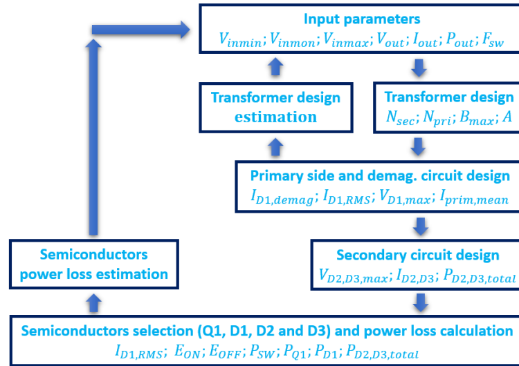
Figure 6. A flow chart illustrating the design process
