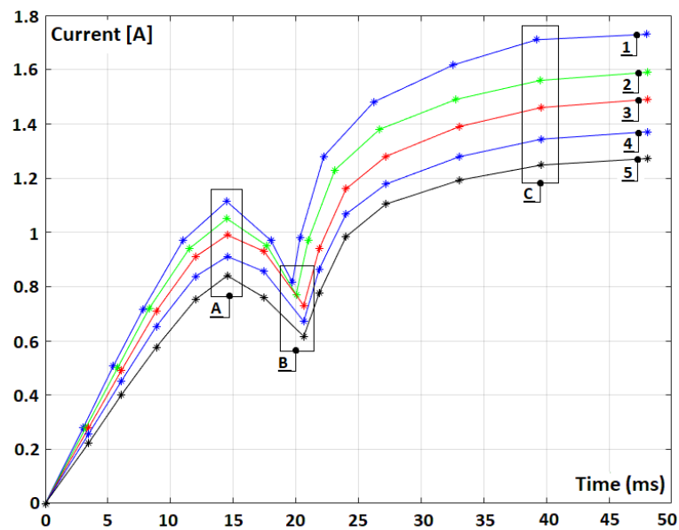
Figure 4. Coil's current variation with the temperature. 1: -10\text{ }^{\circ}\text{C} ; 2: 0\text{ }^{\circ}\text{C} ; 3: 20\text{ }^{\circ}\text{C} ; 4: 40\text{ }^{\circ}\text{C} ; 5: 50\text{ }^{\circ}\text{C} . Section A: variation of the I_{PEAK} ; Section B: variation of the I_{VALLEY} ; Section C: variation of the I_{MAX}
