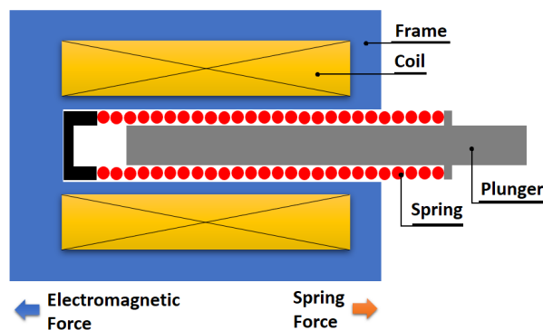
Figure 2. Solenoid electromagnetic system
