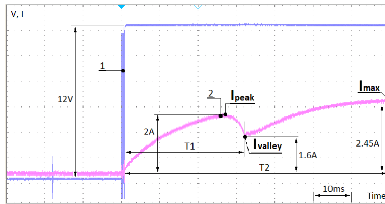
Figure 7. Switching on the transient process of the solenoid. 1- Voltage; 2-Current; T_1 = 17 ms; T_2 = 35 ms; I_{peak} = 2 A; I_{valley} = 1.6 A; I_{max} = 2.45 A
