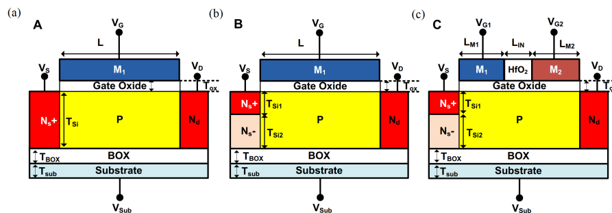
Figure 12. Devices under consideration: (a) conventional FD-SOI MOSFET, (b) referenced FD-SOI MOSFET [15], (c) proposed DMIG Source Engineered FD-SOI MOSFET [18]
