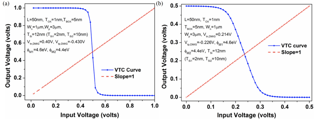
Figure 13. VTC of individual Inverter designed with DMIG FD-SOI MOSFET: (a) at supply voltage = 1 V, (b) at supply voltage = 0.5 V [18]
