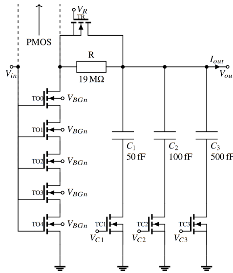
Figure 14. NMOS transistors of one inverter and configurable R and C1 , C2 and C3 [19]
