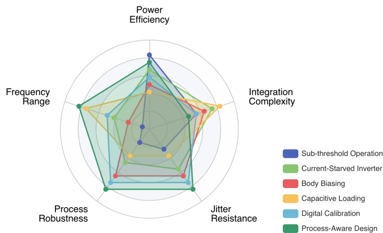
Figure 16. Comparison of ultra-low power Ring Oscillator design techniques across normalized performance metrics
