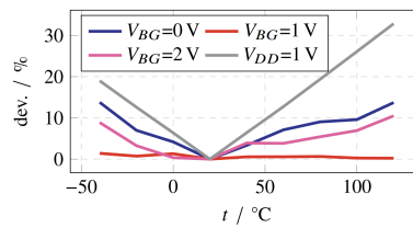
Figure 15. Simulated range of pulse time versus temperature V_{DD}= 0.5 V (colored) compared to V_{DD} = 1 V (Gray) [19]
