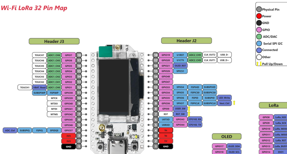
Figure 8. Wi-Fi LoRa 32 V3.2 pin map [12]
