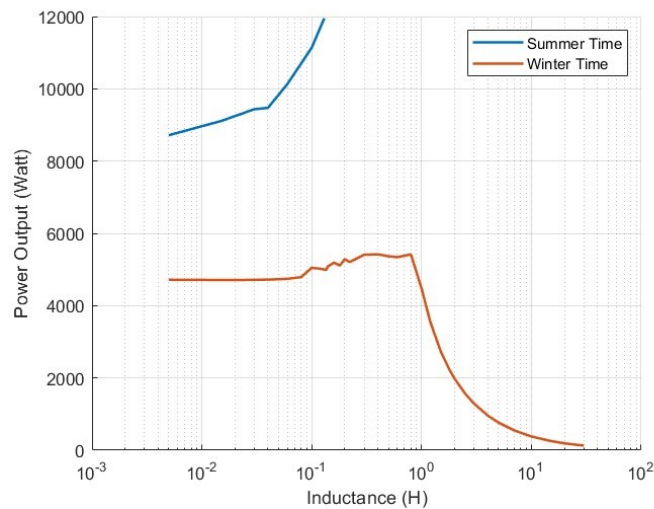
Figure 2. Power output varying inductance
