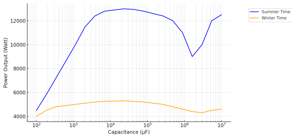
Figure 3. Power output varying capacitance
