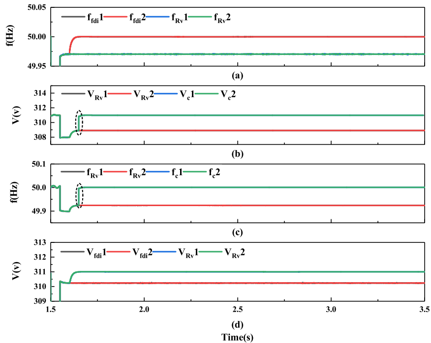
Figure 10. Simulation of adaptive resistive virtual impedance resisting negative constant FDI attack
