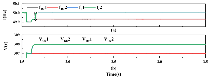
Figure 9. Simulation of adaptive resistive virtual impedance resisting positive constant FDI attack
