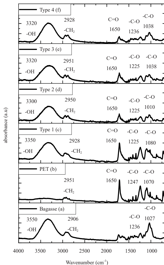
Figure 4. FTIR spectra of (a) Bagasse; (b) PET; (c) Type 1; (d) Type 2; (e) Type 3; (f) Type 4
