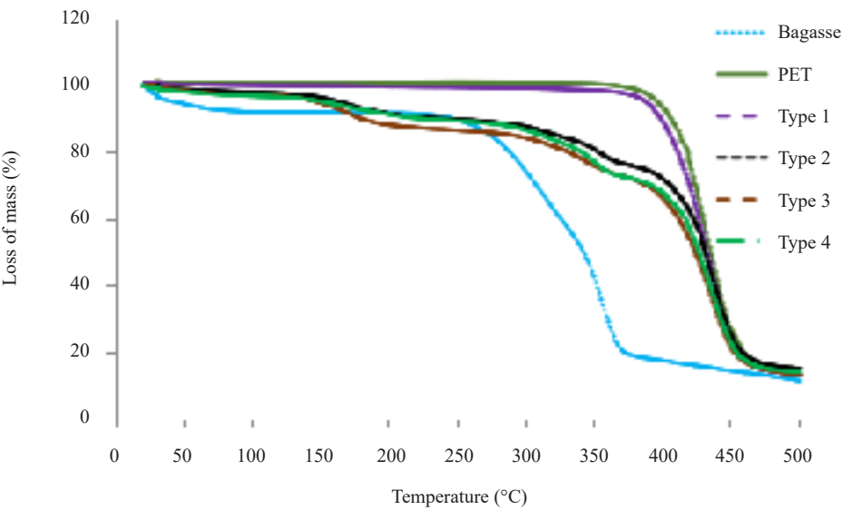
Figure 2. Thermogravimetric analyses of all samples
