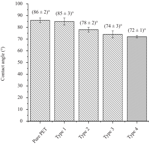
Figure 5. Contact angle
