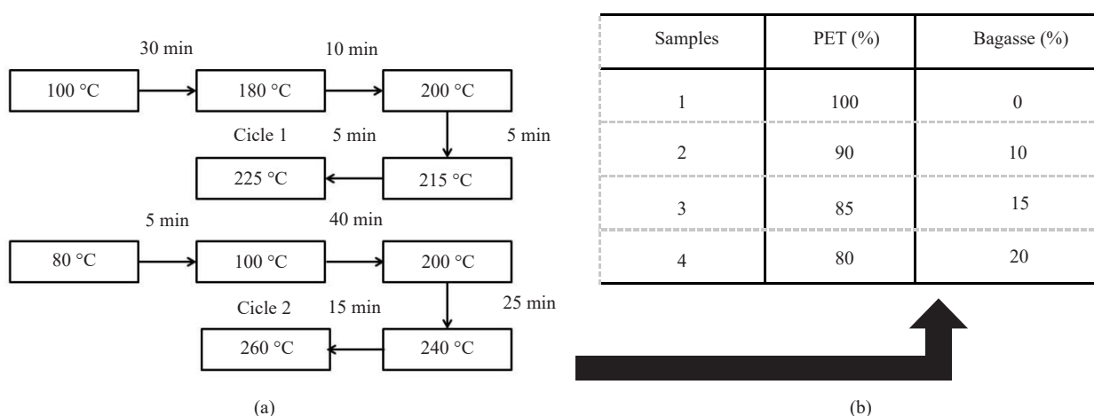
Figure 1. (a) Temperature cycles 1 (PET) and 2 (PET/Bagasse Fiber), (b) Composition of samples
