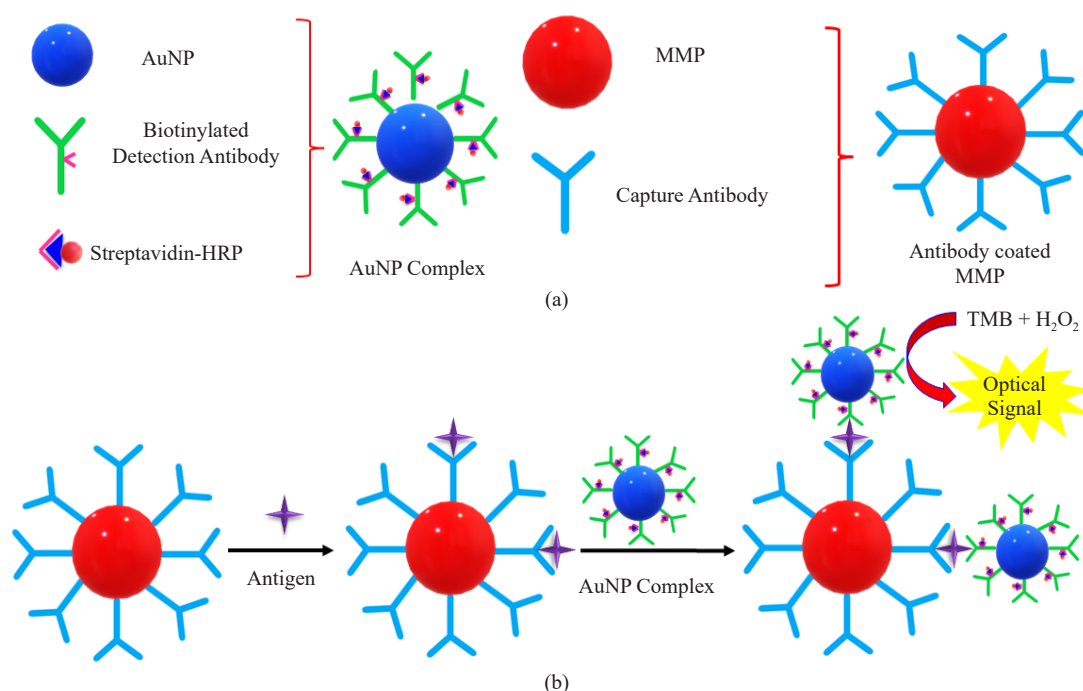
Figure 16. Development of antibody-coated MMP based (a) AuNP-anti-CEA-HRP complex, and (b) AuNP complex based on colorimetric enzyme immunoassay route 66
