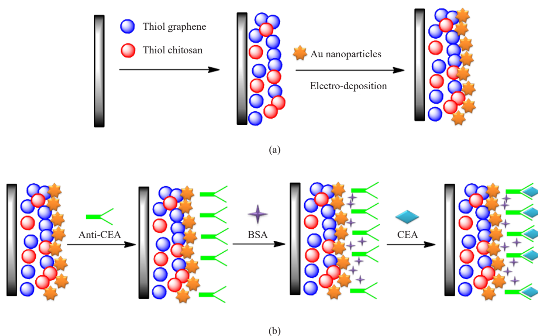
Figure 13. Schematic representation preparation of immunosensor: (a) nanocomposites film, and (b) CEA immunosensor 63
