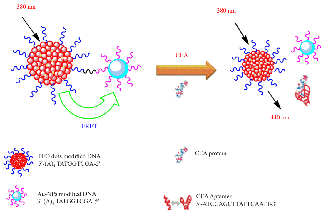
Figure 18. Schematic representation of FRET among PFO dots and Au-NPs for CEA detection 70
