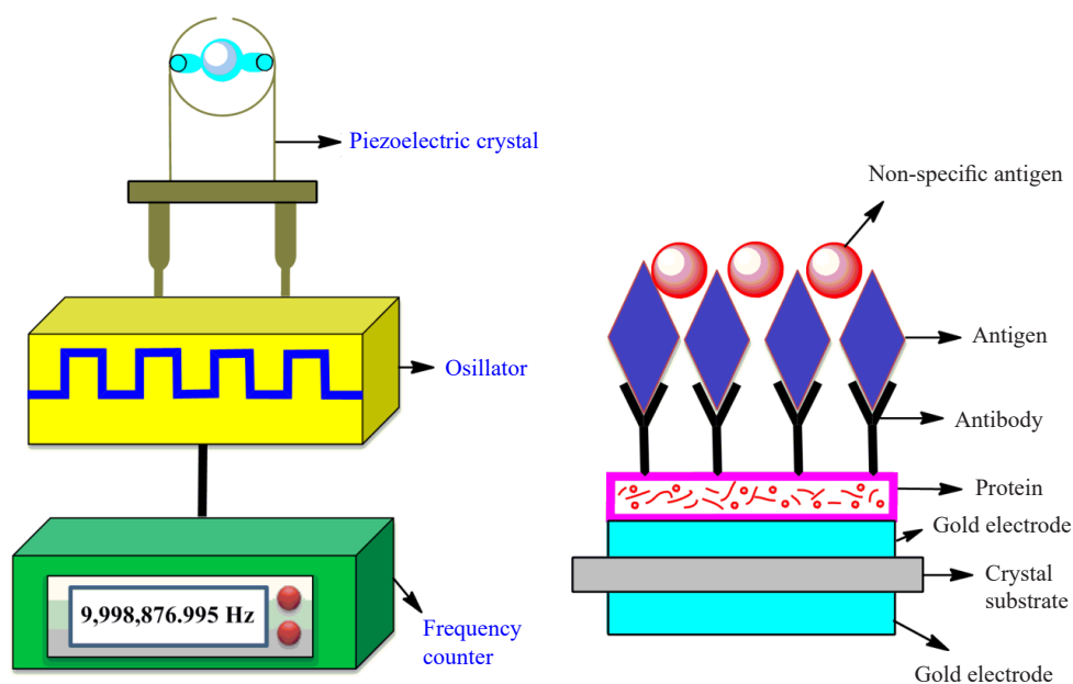
Figure 10. Piezoelectric biosensor demonstrated antibody-antigen binding 58
