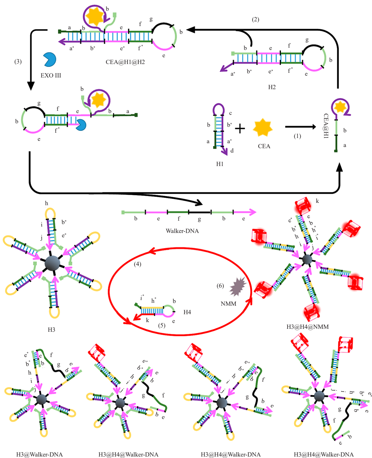
Figure 12. Schematic representation identification of CEA related to the ERA and DNA walker cascade amplification approach, Copyright 2020 ACS 62
