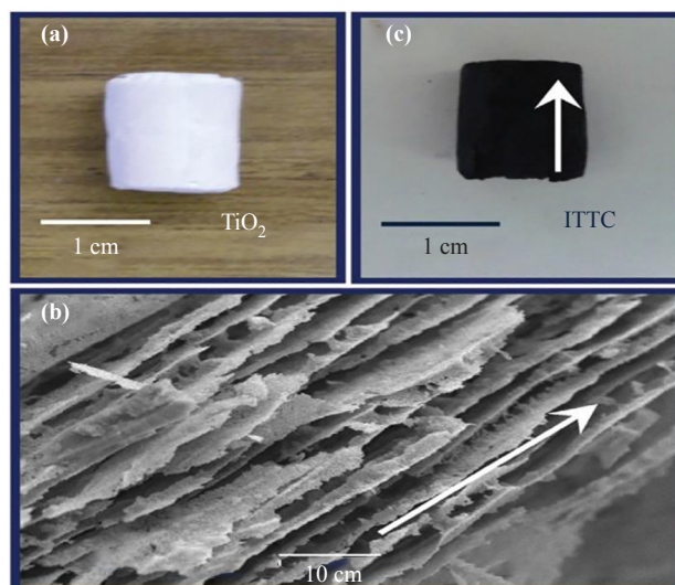
Figure 8. (a) 3\text{DTiO}_2 porous scaffold, precursor of ITTC electrodes, (b) SEM image of the internal architecture of the \text{TiO}_2 scaffold and (c) ITTC electrode obtained by reduction of \text{TiO}_2 porous scaffold 46
