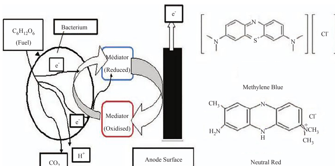
Figure 2. Mediator microbial fuel cell diagram 28
