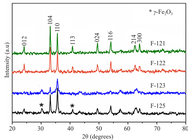
Figure 1. XRD patterns of Fe 2 O 3 samples. F-121 and F-122 belong to \alpha -Fe 2 O 3 phase while F-123 is \gamma phase. F-125 is ( \alpha , \gamma ) mixed phase * represents peaks due to \gamma phase
