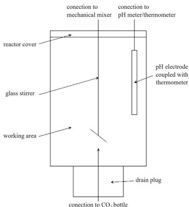
Figure 1. Carbonization reactor
