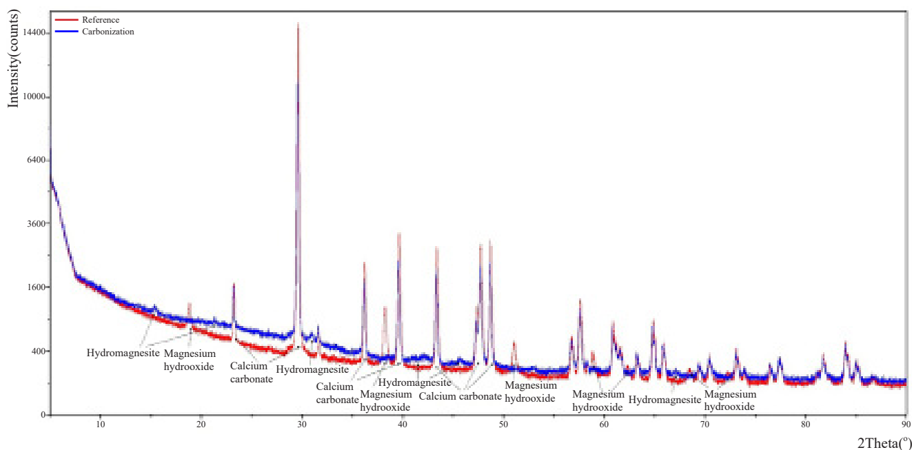
Figure 4. XRD diffractogram
