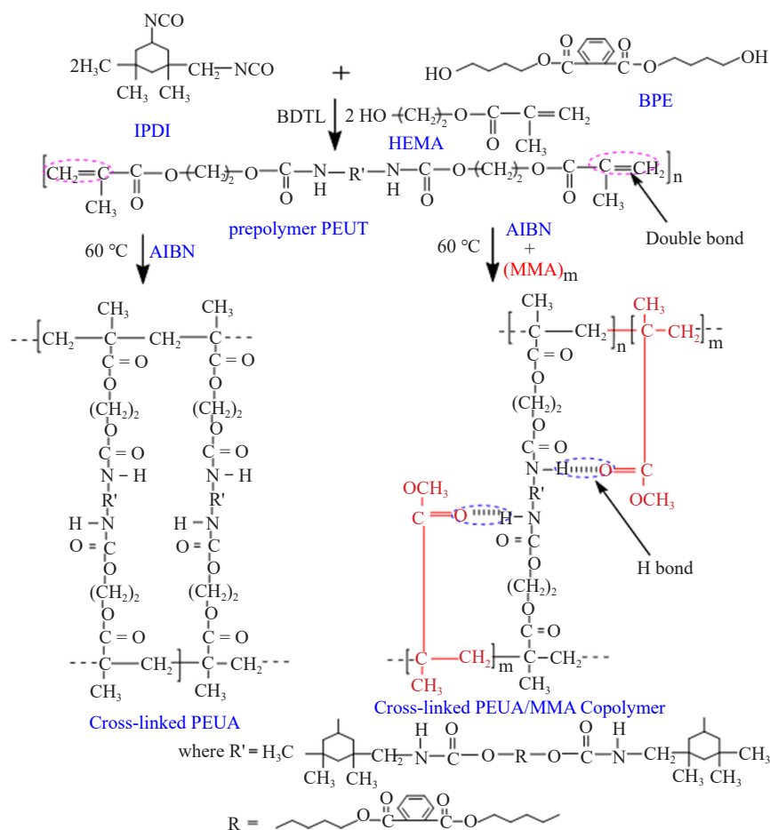
Figure 1. Schematic representation of the synthesis of PEUA and the crosslink structures of PEUA and the PEUA/MMA copolymer
