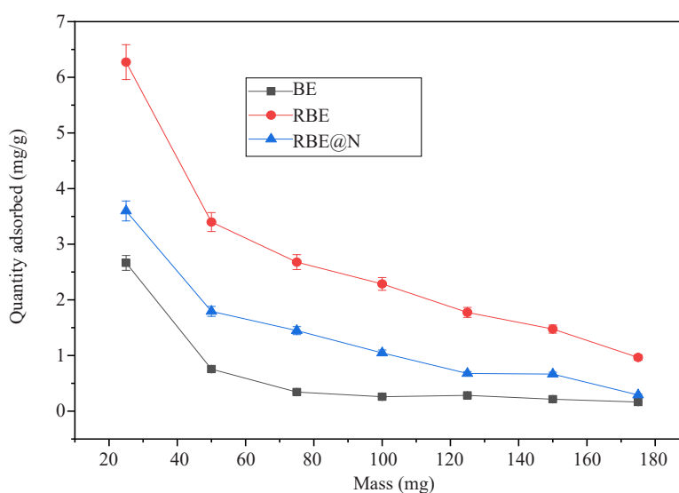
Figure 9. Influence of material dosage on E102 adsorption
