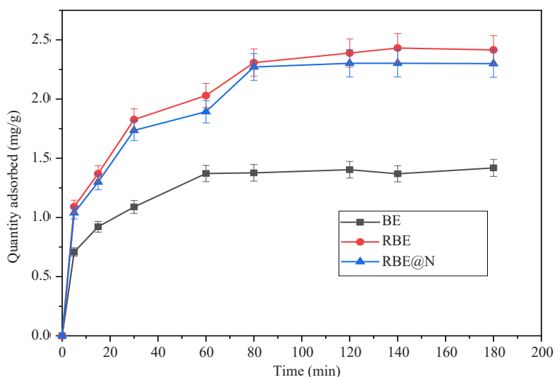
Figure 8. Influence of contact time on the adsorption of E102
