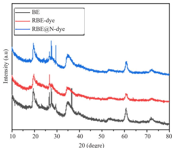
Figure 13. XRD of the materials used after E102 adsorption tests
