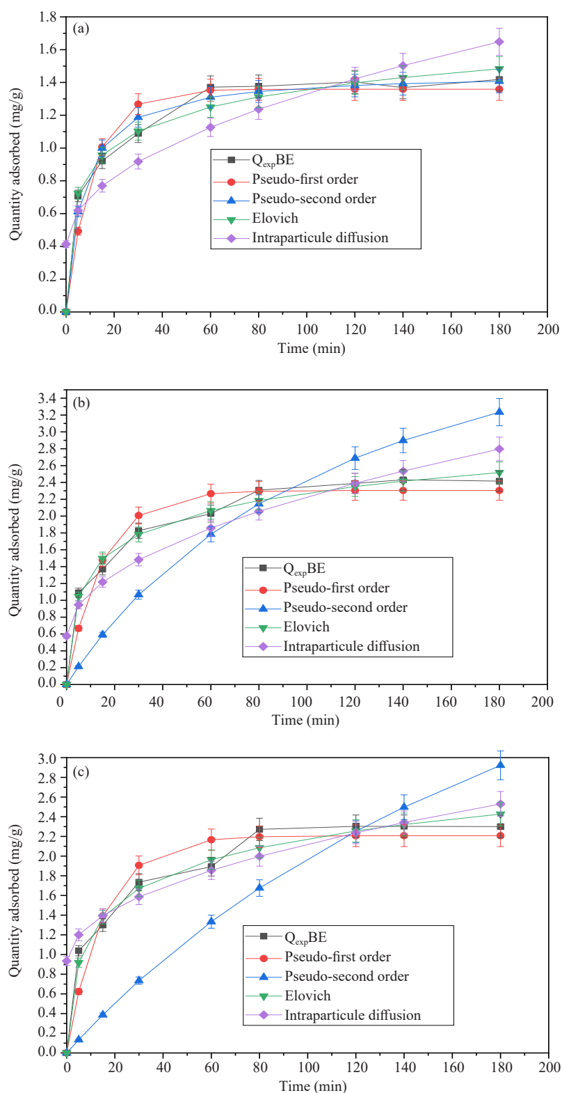
Figure 10. Non-linear forms of kinetic models for (a) BE, (b) RBE and (c) RBE@N
