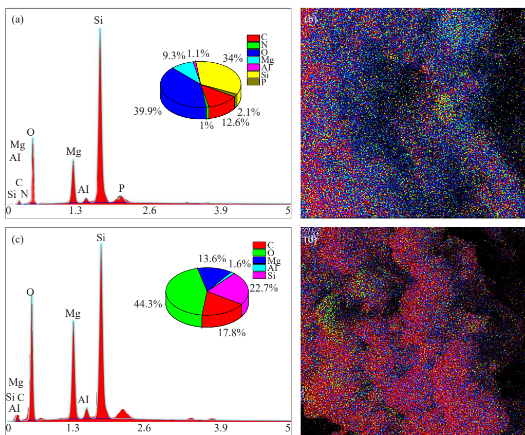
Figure 12. EDX elemental compositions (a), EDX-mapping (b) respectively for the RBE and EDX elemental compositions (c), EDX-mapping (d) element distribution mapping for the RBE@N adsorption of tartrazine
