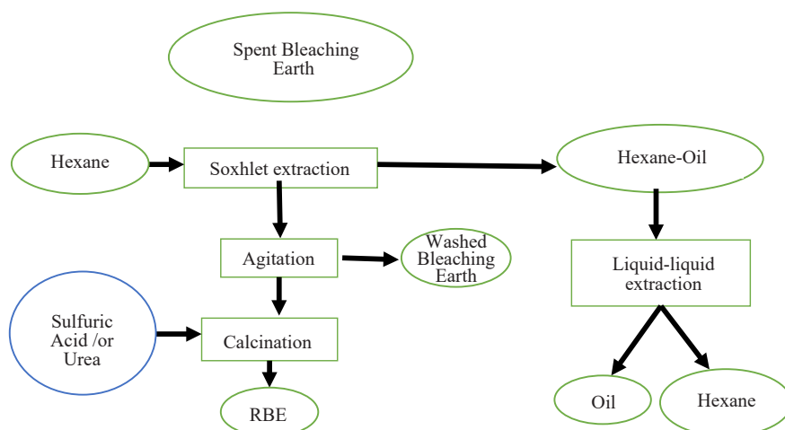
Figure 1. Oil recovery and regeneration of used bleaching earth processes
