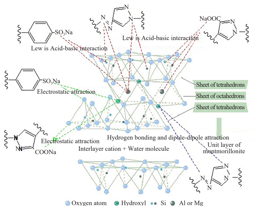
Figure 11. Proposed of adsorption mechanism of tartrazine yellow on different materials
