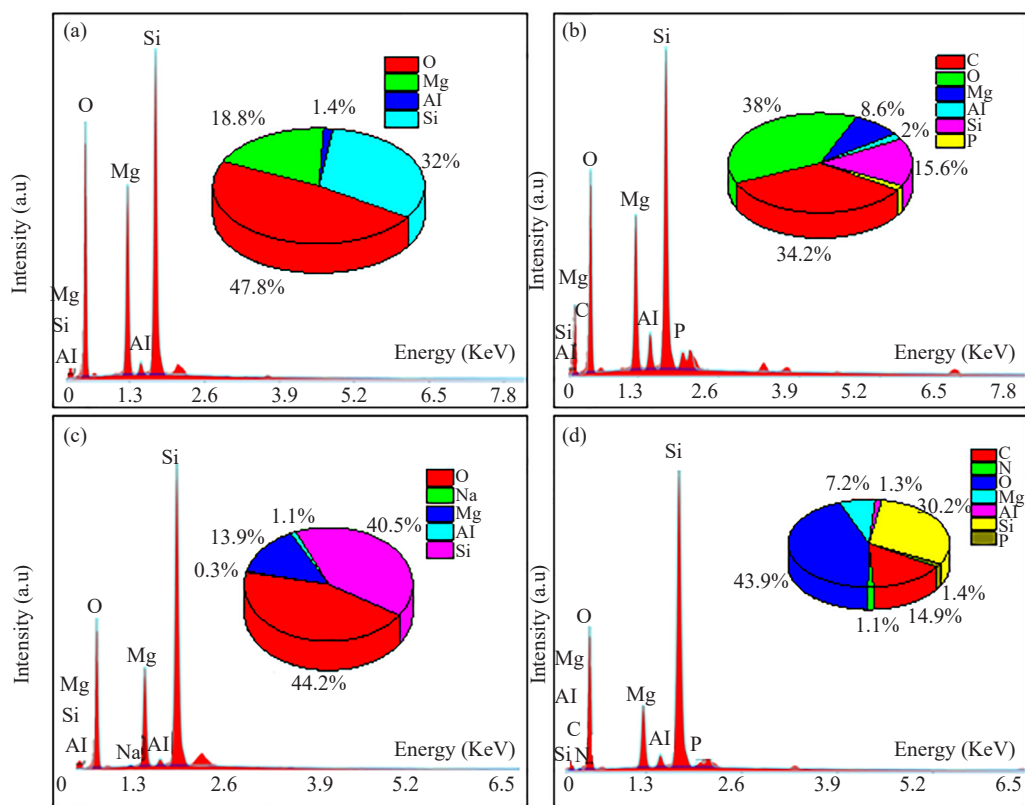
Figure 5. EDX elemental compositions of (a) BE, (b) BE@oil, (c) RBE and (d) RBE@N
