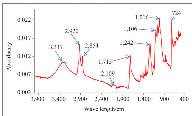
Figure 5. FTIR Analysis of cationized cotton
