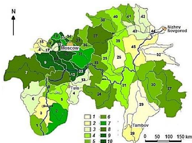
Figure 3. Average values of the indices of elastic-plastic stability of forest formations of the Oka basin (for water-economic areas). 1–45 are the numbers of water supply areas. Indices of the I_{\text{stab}}(i) parameter: 1 – 0.40–0.491; 2 – 0.491–0.506; 3 – 0.506–0.516; 4 – 0.516–0.531; 5 – 0.531–0.549; 6 – 0.549–0.563; 7 – 0.563–0.569; 8 – 0.569–0.597; 9 – 0.597–0.652; 10 – 0.652–0.654
