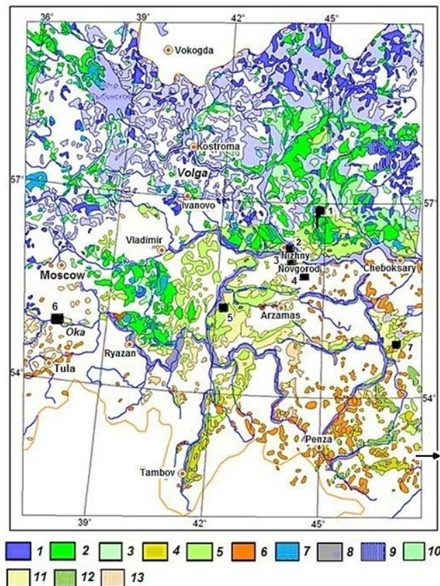
Figure 1. The plant cover of the Middle Volga Region, by [26], and the layout of experimental test sites (calculated and compiled by L.S. Sharaya). 1–13 – convention meanings of plant formations see in the Table 1. Other meanings: 1–8 – test site numbers (explanation in the text)
