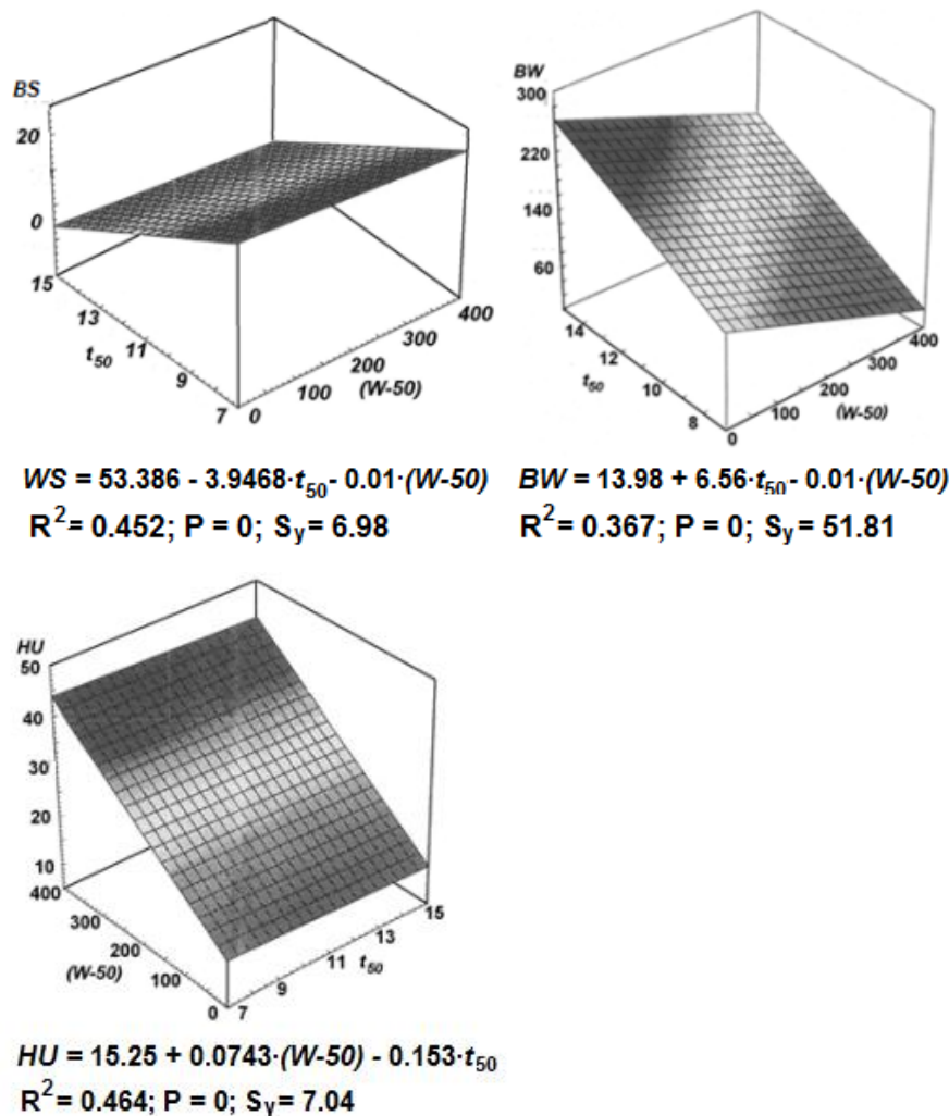
Figure 2. Linear distribution surface of biological cycle parameters in space of soil hydrothermal factors on the mixed forests of the boreal-nemoral forest ecotone, regional ecosystem “Green Town”. Experimental test site 5 (see in the Figure 1)
