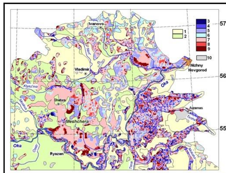
Figure 4. Map of predictive changes of total carbon content on the territory of Oka River basin, by HadCM3 model (calculated and compiled by L.S. Sharaya). The changes in total C stocks for the predicted period of 2100 relative to the base period (t/ha): 3 – (–115) ÷ (–89); 4 – (–89) ÷ (–38); 5 – (–38) ÷ (–12); 6 – (–12) ÷ 0; 7 – 0 ÷ 38; 8 – 38 ÷ 63; 9 – 63 ÷ 15. 1, 2 – fragmentary huge tracts of forest among agricultural fields. 3–9 – forest arias. 10 – the northern area of steppes
