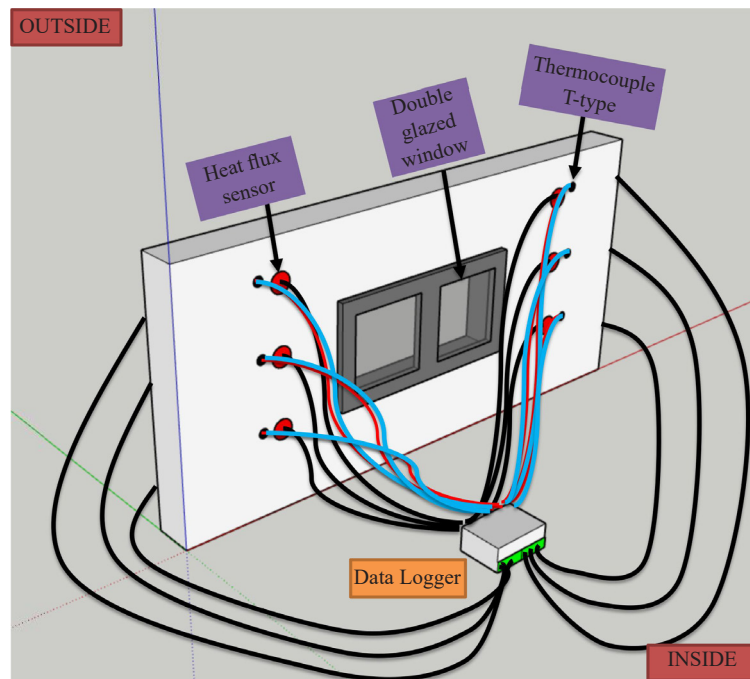
Figure 4. Simply experimental setup demonstration
