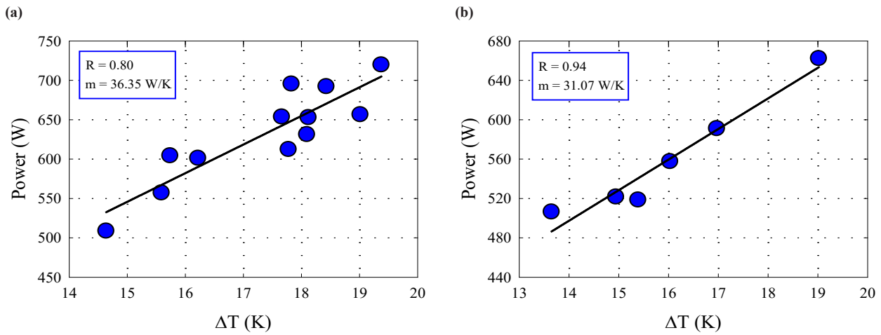
Figure 10. a) Co-heating test for the hall bedroom through regression analysis before the hall bedroom door was closed, b) Co-heating test for the hall bedroom through regression analysis after the hall bedroom door was closed
