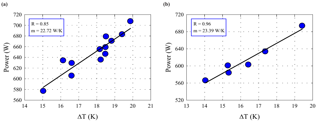
Figure 9. a) Co-heating test for the front bedroom through regression analysis before the test bedroom door was closed, b) Co-heating test for the front bedroom through regression analysis after the test bedroom door was closed
