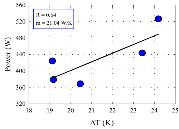
Figure 16. Co-heating test for the back bedroom through regression analysis at the post-retrofitting
