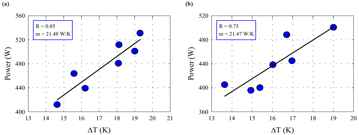
Figure 8. a) Co-heating test for the dining room through regression analysis before the test bedroom door was closed, b) Co-heating test for the dining room through regression analysis after the test bedroom door was closed
