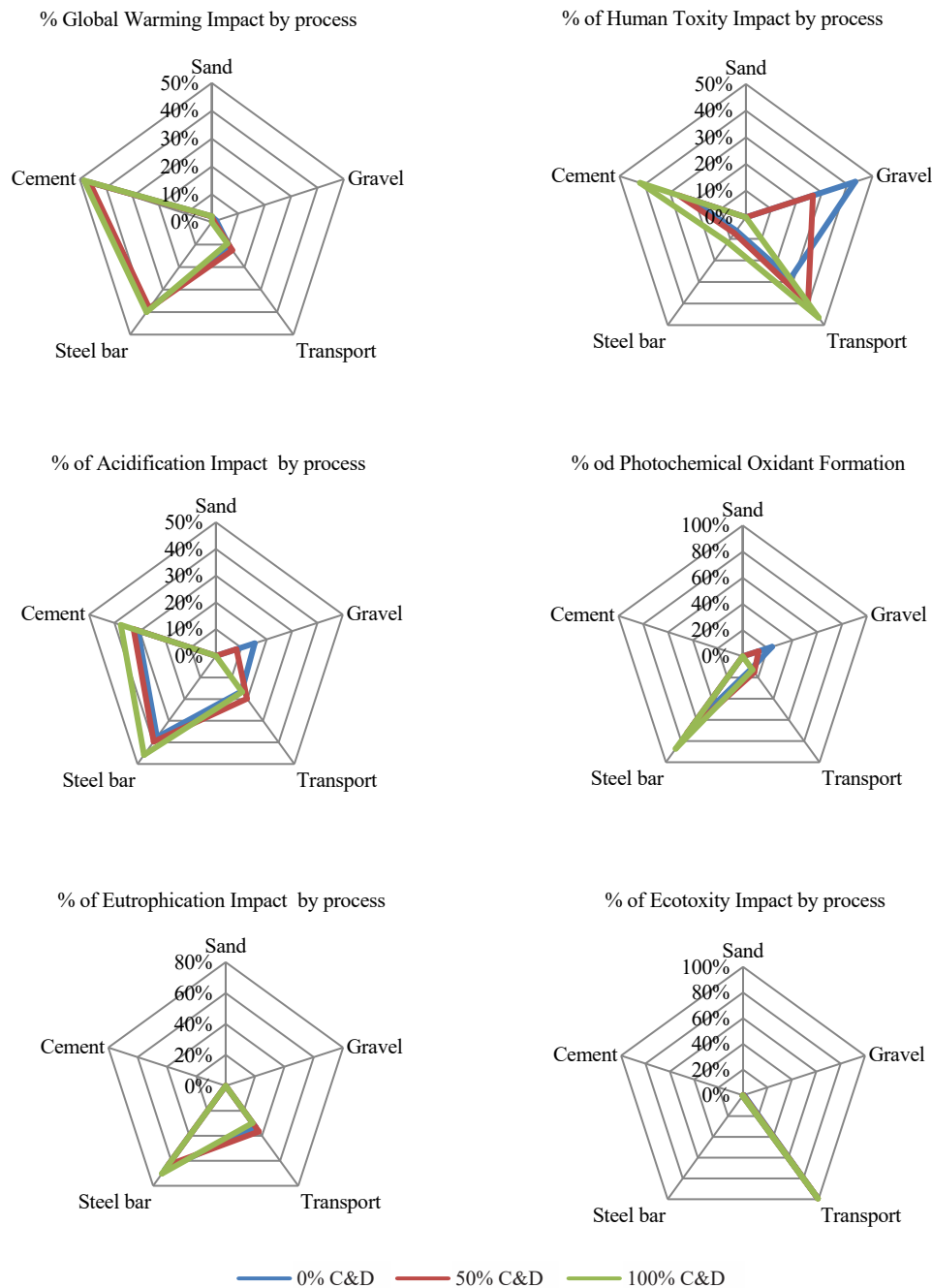
Figure 6. Percentage of Environmental Impact category by production process
