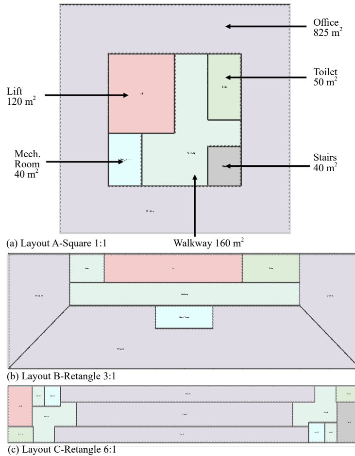
Figure 3. Layout variation for reference office building model
