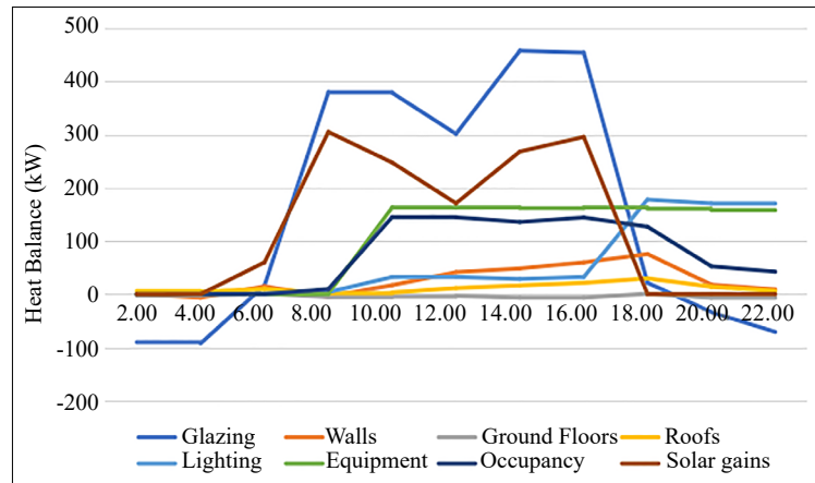
Figure 5. Heat gains and internal gains of the reference building
