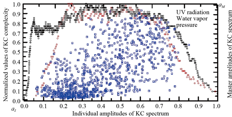
Figure 4. KC spectra of UV radiation (black empty circles) and water vapor pressure (red empty circles). a_M and a_I axes (blue empty squares) in the KC plane, respectively. Daily values of UV radiation for Novi Sad (45° 15' N, 19° 50' E) were obtained from measurements recorded by a broadband Yankee UV-B1 biometer during the period from 2003 to 2005. Daily data on water vapor pressure for the same period were taken from the nearest meteorological station, Rimski Šancevi, which is part of the meteorological network of the Republic Hydrometeorological Service of Serbia and located 8.5 km from the instrument
