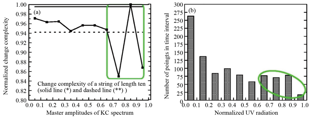
Figure 5. (a) Change in complexity ( CC ) of (i) the master string S_M (*), (ii) the variation of individual strings, and the mean value of change complexity of individual strings S_I (**); (b) dependence of the number of points in a time interval on UV radiation in the time series shown in Figure 3
